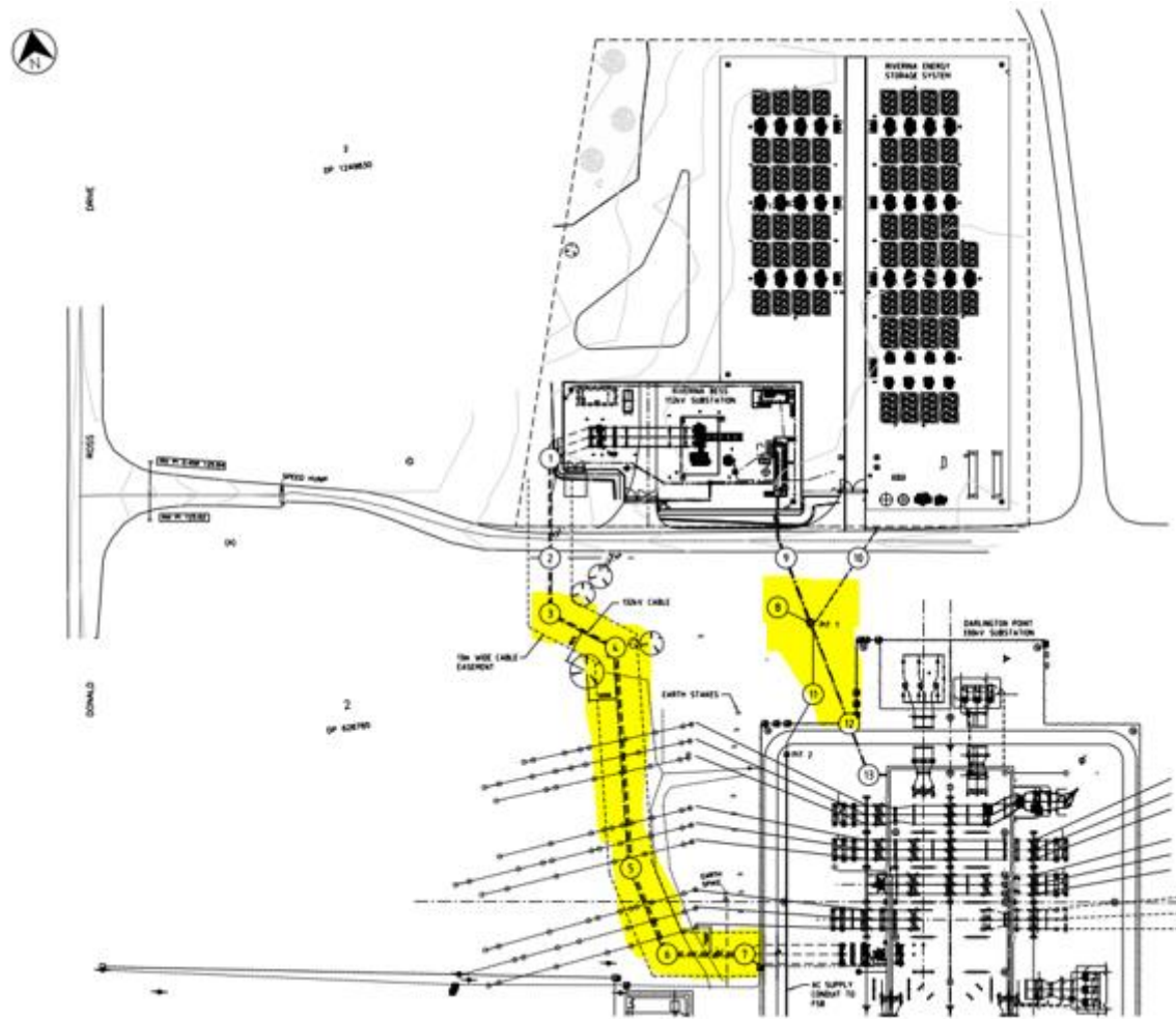
Figure 5: Stage 2b(ii) Connection into the TG DP Sub via 132kV underground cable, control and communications conduits on Lot 2 DP628785 (Project works highlighted in YELLOW)
