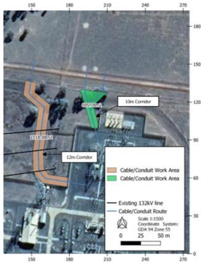
Figure 4: Stage 2b(ii) Detailed Map – 132kV Underground Cable and Conduits connection into the TG DP Sub via 132kV underground cable, control and communication conduits on Lot 2 DP628785
